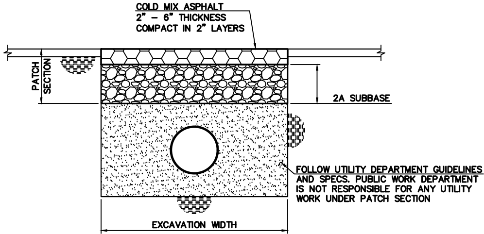
PATCH TYPICAL SECTION
